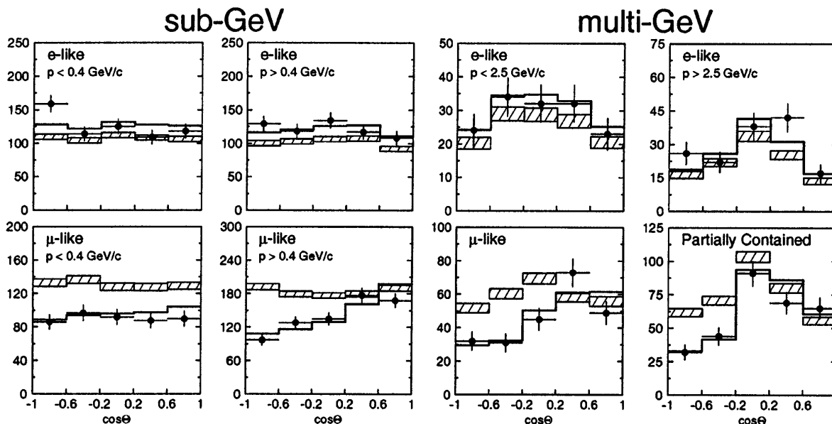
FIG. 3. Zenith angle distributions of \mu -like and e -like events for sub-GeV and multi-GeV data sets. Upward-going particles have \cos \Theta < 0 and downward-going particles have \cos \Theta > 0 . Sub-GeV data are shown separately for p < 400 \text{ MeV}/c and p > 400 \text{ MeV}/c . Multi-GeV e -like distributions are shown for p < 2.5 and p > 2.5 \text{ GeV}/c and the multi-GeV \mu -like are shown separately for FC and PC events. The hatched region shows the Monte Carlo expectation for no oscillations normalized to the data live time with statistical errors. The bold line is the best-fit expectation for \nu_\mu \leftrightarrow \nu_\tau oscillations with the overall flux normalization fitted as a free parameter.
