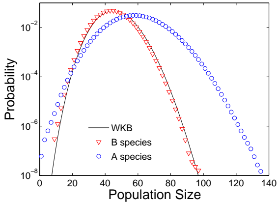
FIG. 2. Quasi-stationary probability distributions for species A, P_m = \sum_n P_{m,n} , and species B, P_n = \sum_m P_{m,n} . Parameters are K = 100 , \epsilon = 0.9 , g = 0.45 , and \alpha = 0 . Symbols are simulation results, while the solid curve is WKB approximation for the B species distribution.
