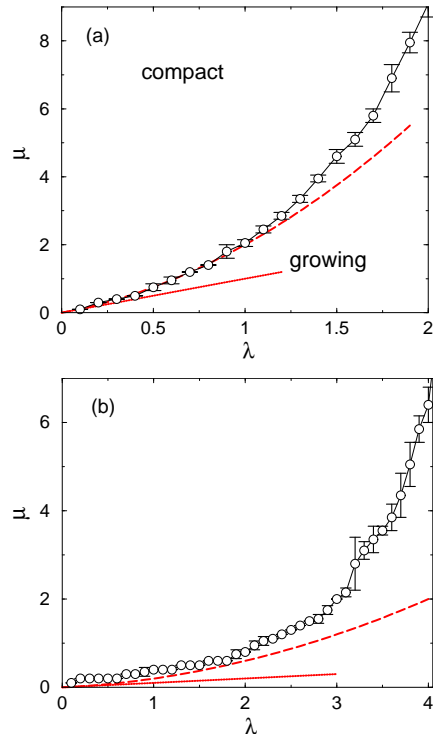
FIG. 6: Phase diagrams of a microtubule from simulations for (a) p = 1 and (b) p = 0.1 . The dashed line represents the prediction (69) that is appropriate for small \mu . The extremes of the error bars are the points for which the tubule velocities are 0.005 and 0.015, and their average defines the data point.
