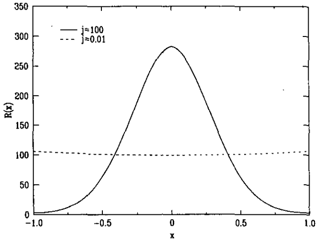
Figure 3. Spatial variation of the local reaction rate R(x) = kc_A(x)c_B(x) in the case of high flux, j = 100 (solid), and low flux, j = 0.01 (dashed). The latter data has been multiplied by a factor of 10,000.
