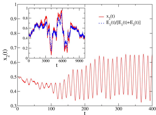
FIG. 2. (Color online) Trajectory of the piston for t < 400 for m_2=100 and initial positions x_1=0.3 , x_2=0.5 , and x_3=0.7636 ; note the offset of the vertical axis. Inset: Trajectory for t < 10^4 , as well as the estimate x_2(t) \approx E_1(t)/[E_1(t)+E_3(t)] (see text). These data are averaged over a 400-point range for ease of visualization.
