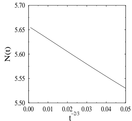
FIG. 1. N(t) versus t^{-2/3} in the subcritical case with b = 0 , b_+ = 1 , b_- = 2 , and \gamma = 0.5 , and with the initial condition P_n(t = 0) = 0.1 for 1 \leq n \leq 10 . The asymptotic intercept with the y axis gives the theoretically predicted value of N_{\min} = 4\sqrt{2} \approx 5.6568 .
