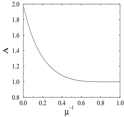
FIG. 2. Average age A of the steady state population versus \mu^{-1} = \sqrt{b_+/b_-} with b = 0 , and with fixed total birth rate equal to one. For \mu^{-1} > 1 , the average age A = 1 , while for \mu^{-1} \rightarrow 0 , A \rightarrow 2 [9].
