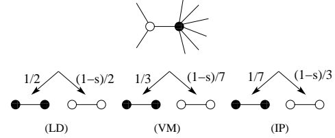
FIG. 1: Update illustration for two specific nodes. Genotypes \mathbf{0} and \mathbf{1} are denoted by \circ and \bullet respectively. Shown are the possible transitions and their respective relative rates due to the interaction of two nodes across a link for LD, VM, and IP dynamics.
