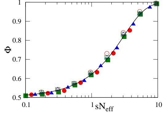
FIG. 3: Scaling plot of fixation probabilities for VM (filled) and IP dynamics (open symbols). Data are for degree-unrelated graphs with N = 10^3 , \mu_1 = 8 , and degree distribution exponent \nu = 2.1 ( \circ ), 2.5 ( \triangle ), or 3.0 ( \square ). Initially each node is a mutant with probability 1/2 , ( \omega_1 = \omega_{-1} = 1/2 ). The curve corresponds to Eqs. (14) or (19).
