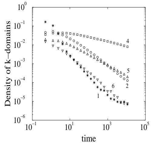
FIG. 2. Density of domains of length 1 (*), 2 (o), 4 ( \square ), 5 ( \Delta ), and 6 ( \nabla ). Simulation results are based on 500 realizations of a chain of 20000 sites with J_3/J_1 > 1 .
