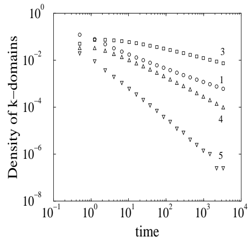
FIG. 1. Density of domains of length 1 ( \circ ), 3 ( \square ), 4 ( \Delta ) and 5 ( \nabla ). Simulation results are based on 1000 realizations of a chain of 20000 sites with J_2/J_1 > 1 .
