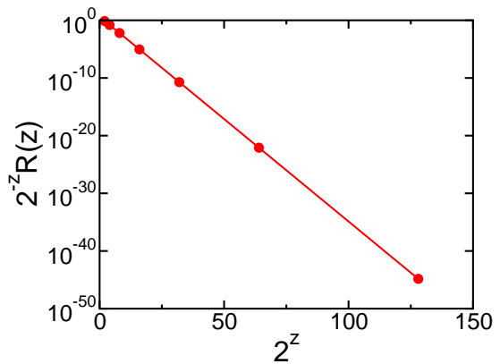
FIG. 7: The super-exponential tail: the quantity 2^{-z}R(z) versus 2^z , obtained by numerical integration of (25) to time t = 100 with r = 0 .
