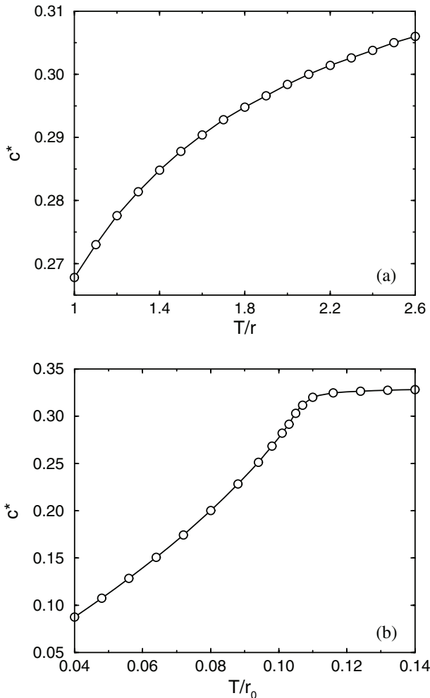
Fig. 3: Simulation results for the fixed point minority concentration c^* for: (a) a population of N = 5000 agents with constant strategic bias as a function of x = \frac{T}{r} , and (b) N = 50000 agents with state-dependent strategic bias as a function of x_0 = \frac{T}{r_0} . The numerical value c^* , which agrees perfectly with the rate equation predictions, is determined by the time integral of the concentration divided by the observation time. The change in behavior when x_0 \approx \frac{1}{9} becomes a cusp as N \rightarrow \infty .
