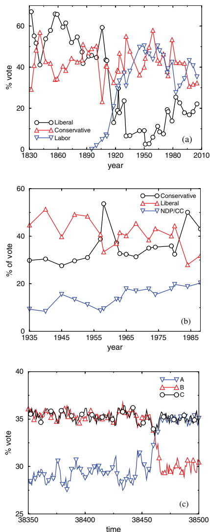
Fig. 1: (a) British election results since 1830. (b) Canadian election results from 1935–90; here NDP/CC denotes the New Democratic Party and its Cooperative Commonwealth party antecedent. (c) Representative simulation results for the time evolution of the densities of the three states in the strategic voter model with state-dependent strategic bias for 50000 agents and parameter x_0 = 0.104 (see text for definition of x_0 ).
