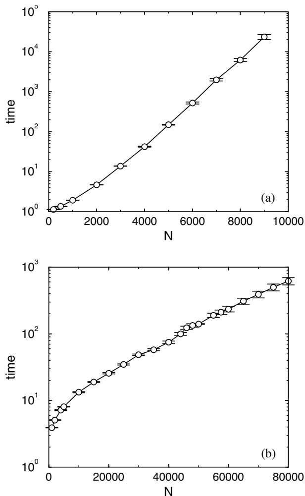
Fig. 4: Average time span for a single party to have minority status vs. population N for strategic voting with: (a) constant strategic bias with x = 2 and (b) state-dependent strategic bias with x_0 = 0.104 ; this latter value is chosen to give the same steady-state minority densities for both models. Both time dependences are consistent with exponential growth in N .
