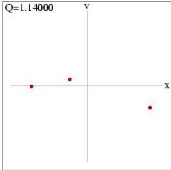
Periodic motion
