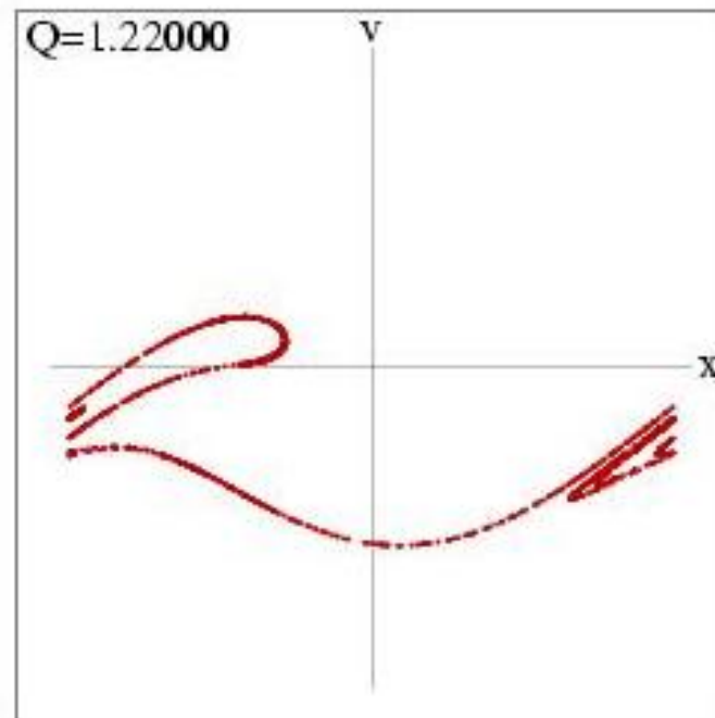
chaotic motion
