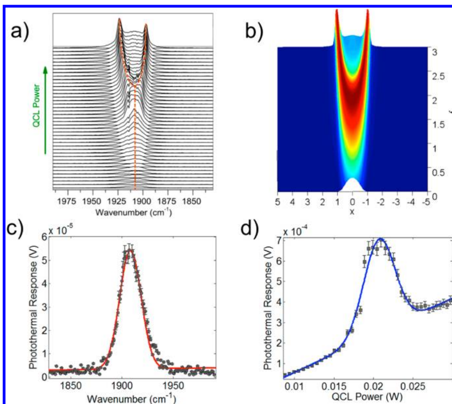
Figure 2. (a) Linear and nonlinear regimes in Photothermal IR spectroscopy in 8CB at 29 °C. Spectra have been displaced vertically for clarity. At small QCL current, the photothermal spectrum closely follows the linear FTIR spectrum. At high currents, the spectrum indicates a bifurcation. The critical power at the peak frequency is at incident QCL power of 0.021 W. (b) Surface plot of the calculated photothermal signal S_{\text{Tot}} using the phenomenological model described in the paper. The scaled dimensionless QCL frequency x and the scaled dimensionless QCL power y are defined in the text. (c) Photothermal response at a low incident pump power of 0.01 W, where the response is still in the linear regime. Solid line is a fit to a Gaussian function in frequency with a fwhm 37 \pm 2 cm -1 . (d) Photothermal response above the bifurcation transition for 29 °C, as a function of incident infrared power P , for a fixed frequency at the peak of the IR absorption band 1912 cm -1 . The solid line is a fit to a term linear in the power to represent the linear response and a Gaussian form for the nonlinear component, as described in the text.
