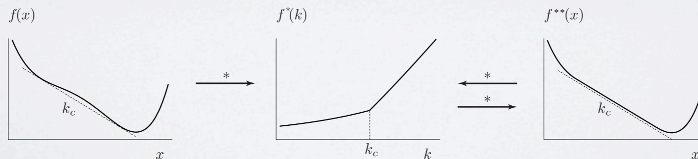
Figure 8: Structure of the LF transform for nonconvex functions.
