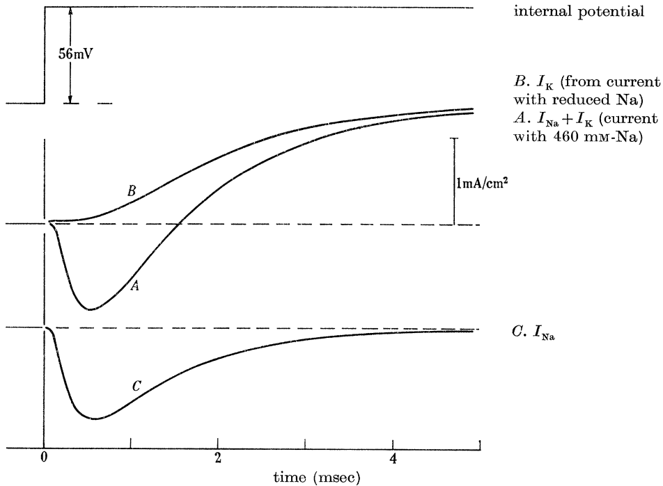
FIGURE 9. Separation of current into components carried by Na and K, from Hodgkin & Huxley (1952 a , figure 5). A depolarization of 56 mV was applied at t=0 ; the temperature was 8.5^\circ\text{C} . Outward current is shown upwards.
