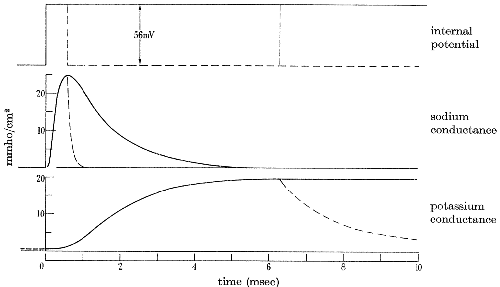
FIGURE 10. Changes in sodium and potassium conductance associated with depolarization of 56 mV, applied at t=0 ; temperature 8.5^\circ\text{C} . The continuous curves, which were obtained from the experiment of figure 9, show the changes in conductance when the depolarization was maintained; the broken curves, which were drawn from data obtained in other experiments, give the effect of repolarizing the fibre after 0.6 or 6.3 msec. From Hodgkin & Huxley (1952 a , b, d).
