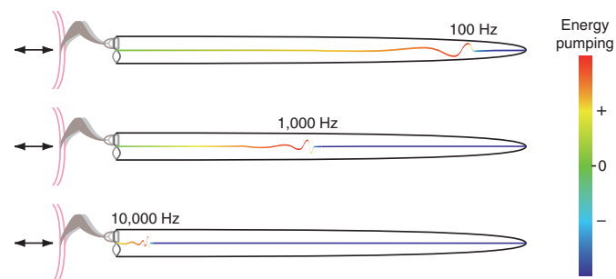
FIG. 3. Locus of energy pumping on the basilar membrane. Each of the 3 diagrams portrays the instantaneous position of the basilar membrane during the propagation of a traveling wave of the indicated frequency. The color scale portrays the extent of energy pumping. The active process grows progressively stronger as the wave approaches the characteristic place, then declines rapidly just before the resonant position associated with the stimulus frequency. If the traveling wave were capable of propagating farther apically than the resonant position, the active process would withdraw energy from it. Note that the amplitude of the traveling wave has been exaggerated about 10^5 -fold with respect to the length of the basilar membrane.
