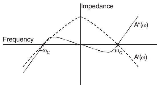
FIG. A1. Schematic representation of the impedance A(\omega) = A'(\omega) + iA''(\omega) of a critical oscillator as a function of the stimulus frequency \omega . In the linear limit of cochlear mechanics, the local impedance A of the cochlear partition is defined as the ratio of the Fourier component of the cross-sectional pressure to the Fourier component of the basilar-membrane vibration at the frequency of stimulation. This impedance is a complex number with units of stiffness per unit area. The real or reactive part A' is an even function of \omega , whereas the imaginary or dissipative part A'' is odd. Criticality requires that the impedance vanish at \omega = \pm\omega_c , in which \omega_c is the characteristic frequency of the oscillator. At low frequencies, as A'' approaches zero, A' > 0 describes the local stiffness of the cochlear partition. At high frequencies, A' < 0 is instead dominated by inertia, whereas A'' > 0 reflects dissipation by hydrodynamic friction. These generic constraints ensure that a critical oscillator provides net negative damping ( A'' < 0 )—corresponding to the active pumping of energy into the traveling wave—when stimulated below its characteristic frequency, but that it dissipates energy ( A'' > 0 ) when stimulated above that frequency. Note that energy pumping peaks at a frequency below \omega_c . In principle, an active oscillator may also achieve criticality by opposing damping so that A'' = 0 at all frequencies (APPENDIX B). This is the case for the van der Pol oscillator, a standard model for the generation of spontaneous oscillations (Strogatz 1994). However, this singular realization of a critical oscillator does not produce energy pumping.
