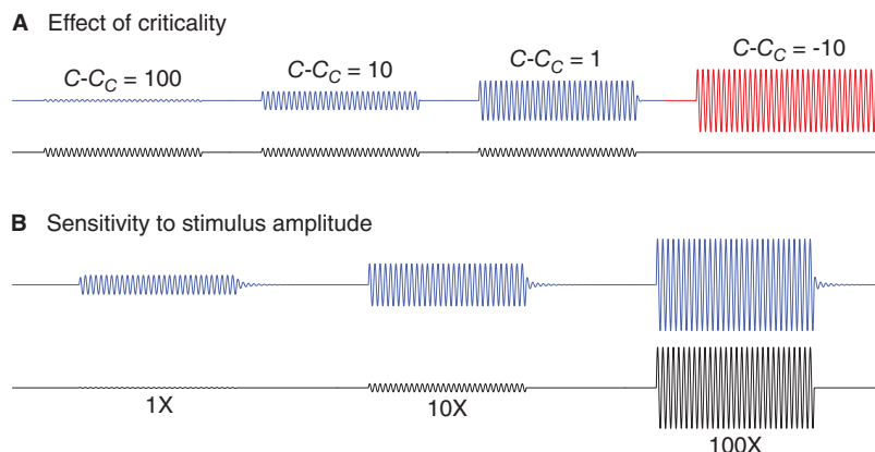
FIG. 1. The behavior of a critical oscillator. A: an oscillator whose response is described by Eq. 1 produces sinusoidal responses (top traces) when driven at its characteristic frequency with pulses of sinusoidal stimuli (bottom traces). As the difference between the value of the control parameter and the critical value, C - C_c , declines from 100 to 10 and then to 1, the response to identical stimuli grows substantially. Finally, when C - C_c = -10 , the system becomes unstable and undergoes limit-cycle oscillation in the absence of stimulation. B: when the oscillator operates near criticality, here with C - C_c = 0.1 in each panel, its response exhibits compressive nonlinearity. As the stimulus grows by successive factors of 10, the responses increase by factors of only 10^{1/3} or about 2.2.
