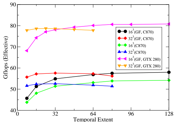
Figure 3: Performance of the conjugate gradient inverter.
