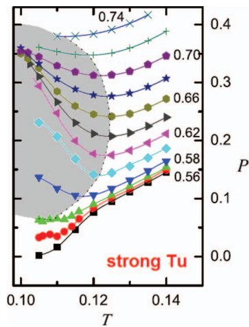
FIG. 5. Isochores of the Tu model for the strong tetrahedrality version, which has a LLCP. 34 Gray area indicates the density anomaly region. By reducing the tetrahedrality, the Tu model can be smoothly changed into the weak tetrahedrality version, which does not have a LLCP. The isochores of WAC (Fig. 1(b)) show no LLCP but closely resembles that of the strong Tu model. We can interpret this as that WAC is close to having a LLCP, but not close enough. If we were to enhance the tetrahedrality of WAC, it is likely a LLCP would appear.
