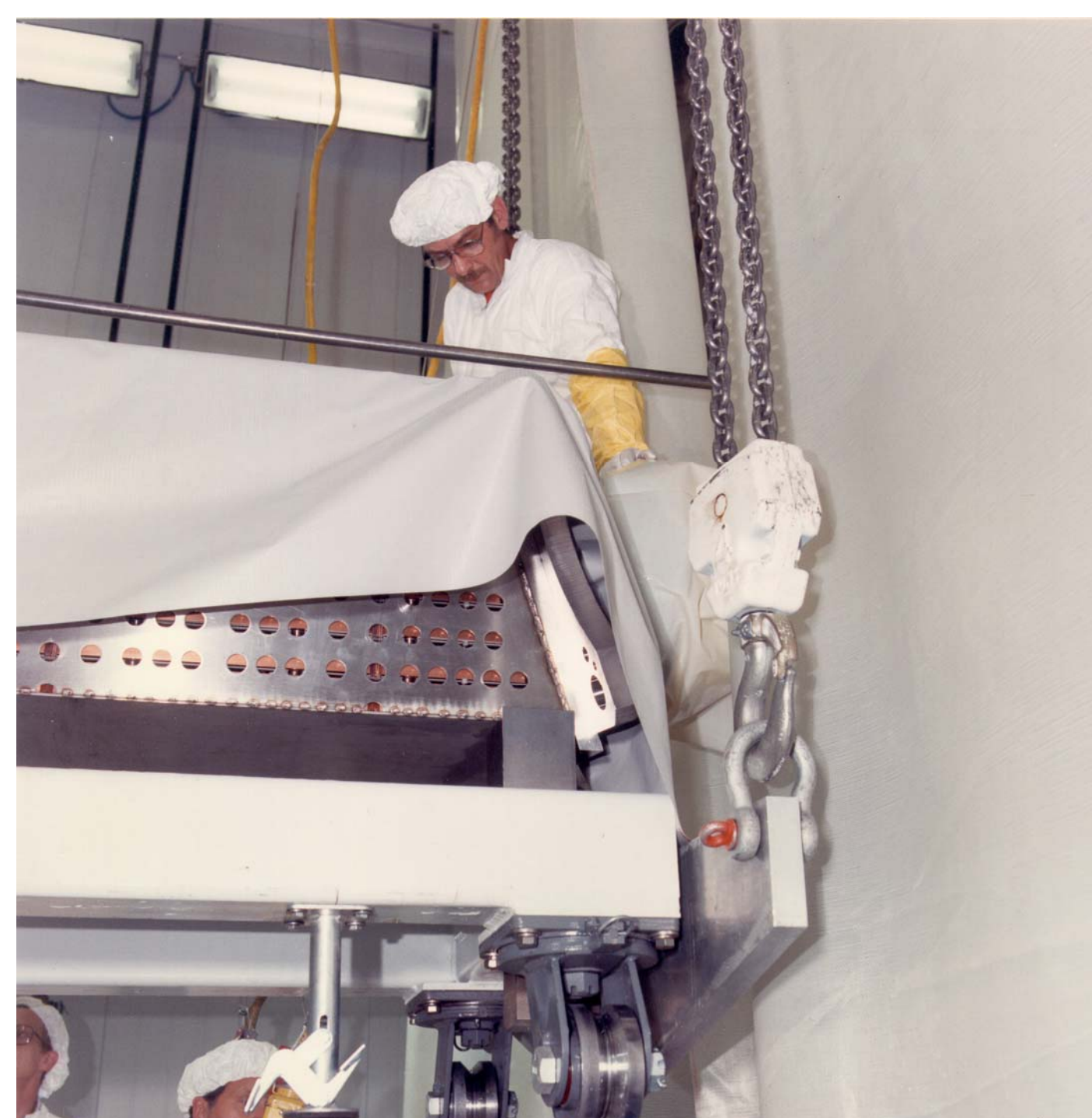
Joe Morrison preparing to lift a module to the C-frame for installation
