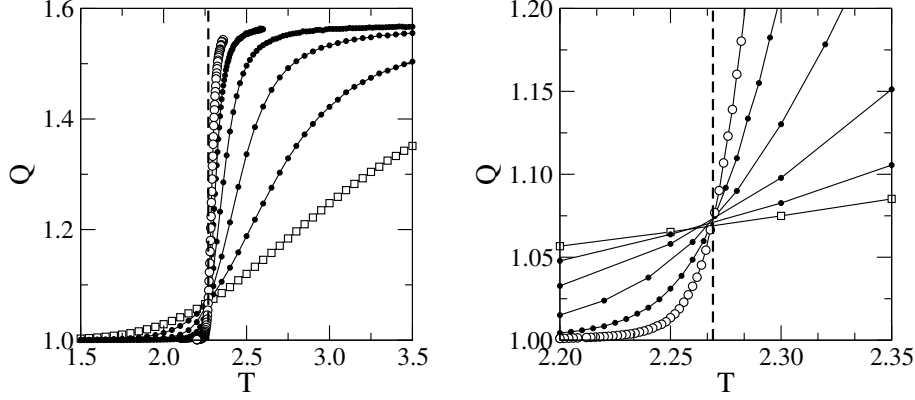
Figure 20: Binder ratio for the 2D Ising model with L = 4 (open squares), 8, 16, 32, 64, and 128 (open circles) graphed using two different scales. The dashed lines indicate T_c .
