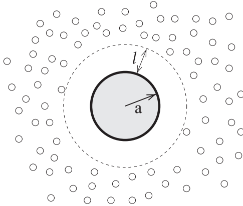
Figure 1. Model geometry in two dimensions. A gas of density \rho occupies the region r > a+l exterior to a circular absorber centered at the origin.
