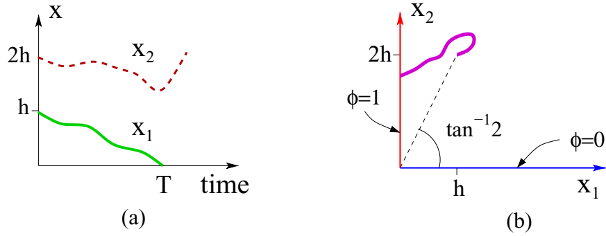
Figure 4. Correspondence between (a) two particles diffusing on the positive half line and (b) an effective particle, with coordinates x_1 and x_2 , diffusing in the positive quadrant in two dimensions.
