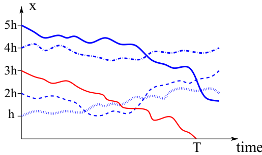
Figure 3. Illustration of hitting in one dimension. Particles are initially at x = h, 2h, 3h, \dots . The first particle (here particle 3) hits the absorber at time T .
