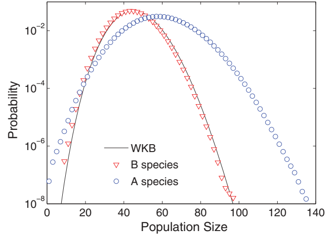
FIG. 2. (Color online) Quasistationary probability distributions for species A , P_m = \sum_n P_{m,n} , and species B , P_n = \sum_m P_{m,n} . Parameters are K = 100 , \epsilon = 0.9 , g = 0.45 , and \alpha = 0 . Symbols are simulation results, while the solid curve is WKB approximation for the B species distribution.
