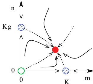
FIG. 1. (Color online) Schematic flow diagram in asymmetric two-species competition for weak competition in the mean field. The unstable node, the saddles, and the stable node are shown as open, hatched, and solid, respectively.
