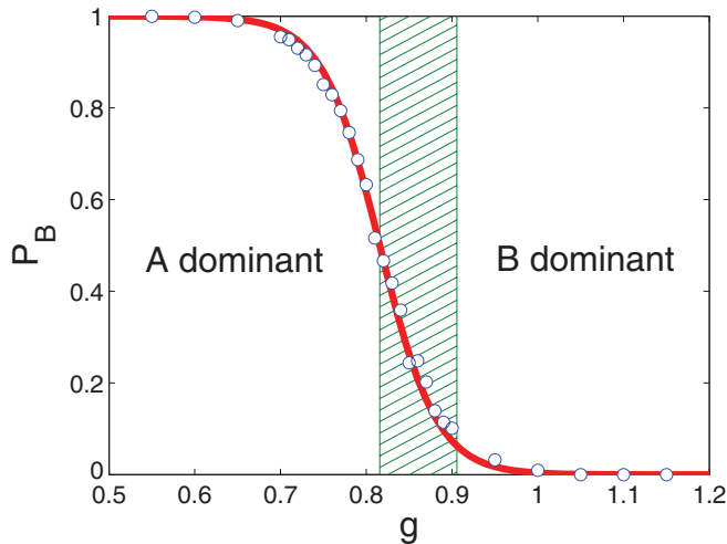
FIG. 3. (Color online) Probability that species B first becomes extinct as a function of growth rate asymmetry g for \alpha = 0 , \epsilon = 0.1 , and K = 40 . The curve is the prediction of Eq. (14), with actions given by (19), while circles are simulation results. In the hatched region, the quasistationary population of B is less than that of A , but B 's are less likely to become extinct first.
