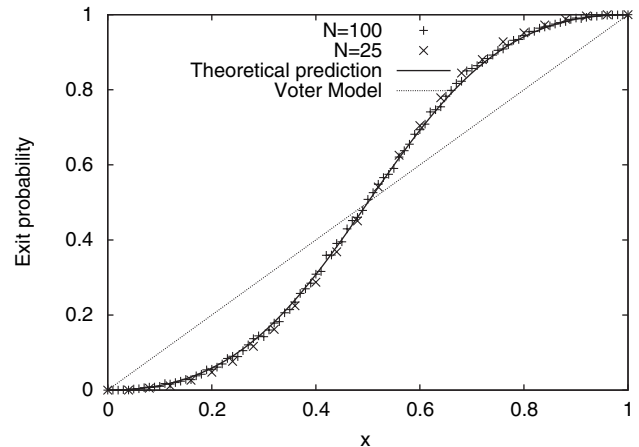
Fig. 4: Exit probability \mathcal{E}(x) for the Sznajd model. The system is one dimensional and composed of 25 and 100 voters, respectively. Results are averaged over 5000 realizations of the random process.
