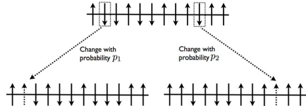
Fig. 1: Update illustration. A random voter changes state with probability p_1 if it has 1 disagreeing neighbor (left), and with probability p_2 if it has 2 disagreeing neighbors (right).
