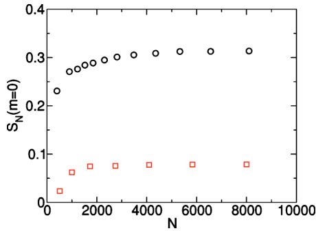
FIG. 8. Probability to reach a stripe state versus number of spins N for d=2 ( \circ ) and d=3 ( \square ) using the threshold value 0.5 (see text). Data are based on 10^5 realizations.
