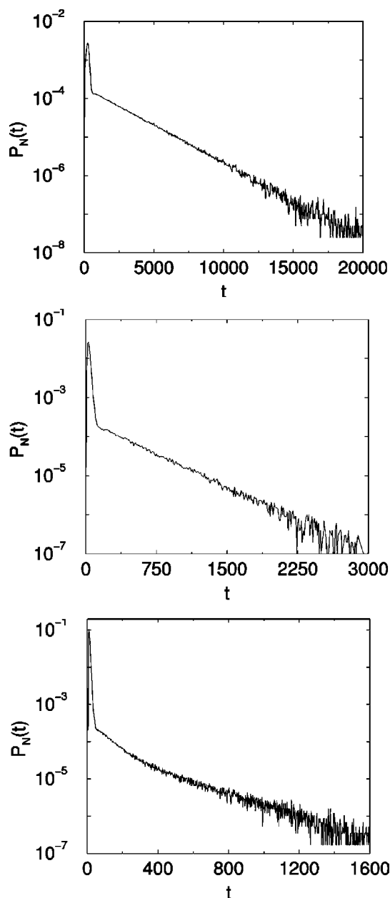
FIG. 2. Distribution of consensus times, P_N(t) , versus t (in units of Monte Carlo steps per spin) for an N -spin system starting from a random zero-magnetization state. Shown are results for (top to bottom) a 50^2 square lattice ( N=2500 ), a 14^3 cubic lattice ( N=2744 ), and a 7^4 four-dimensional hypercubic lattice ( N=2401 ). Data are all based on 10^6 realizations.
