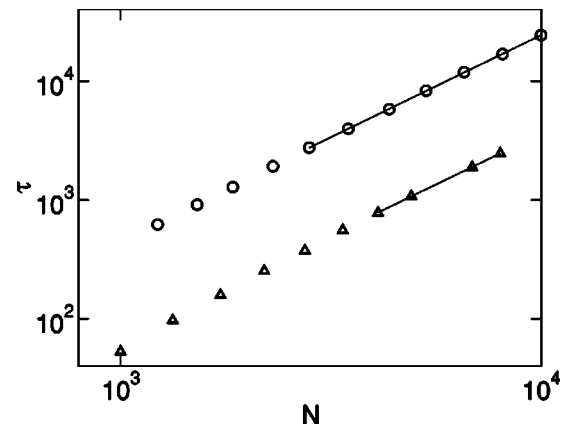
FIG. 4. Double logarithmic plot of \tau(N) (in units of Monte Carlo steps per spin) versus N for d=2 ( \circ ) and d=3 ( \triangle ). The lines are the best fits to the last few data points.
