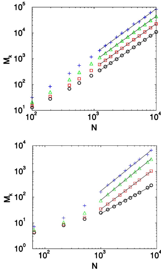
FIG. 3. Double logarithmic plot of M_k(N) , the k th reduced moments of the consensus time distribution, versus the total number of spins N for k=1 ( \circ ), k=2 ( \square ), k=4 ( \triangle ), k=8 ( + ), in d=2 (top) and d=3 (bottom). Data are based on 10^5 realizations in d=2 and 4 \times 10^5 realizations in d=3 . The lines are least-squares linear fits to the large- N data.
