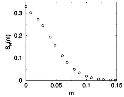
FIG. 9. Probability to reach a stripe state versus initial magnetization m for a 50^2 system. Data are based on 10^5 realizations.
