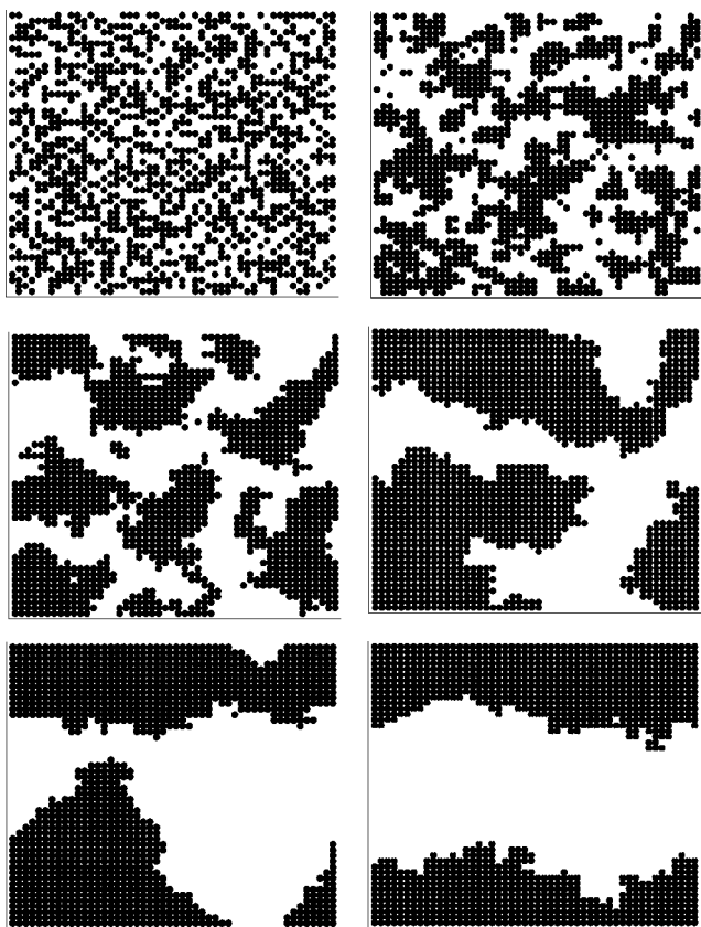
FIG. 5. Snapshots of a 50^2 system at t=0, 1, 5, 20, 80, and 200 .
