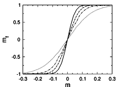
FIG. 10. Final magnetization m_f as a function of initial magnetization m , on the square lattice for linear dimension L=10 (dotted curve), 20 (dashed), 30 (dot-dash), and 50 (solid).
