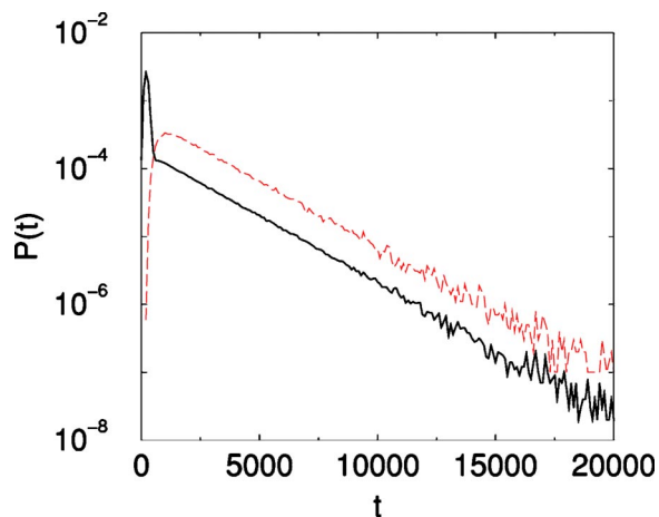
FIG. 7. Consensus time distribution for a 50^2 square lattice for a two-stripe (dashed) and random initial condition (solid). All data are based on 10^5 realizations. Time is in units of Monte Carlo steps per spin.
