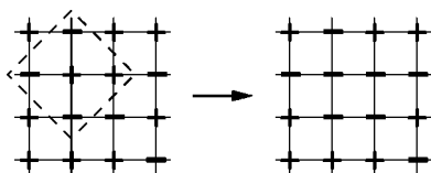
FIG. 1. Illustration of a single majority rule update step for the five-site von Neumann neighborhood on the square lattice.
