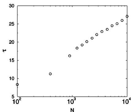
FIG. 11. Consensus time (in units of Monte Carlo steps per spin) versus N in d=2 for initial magnetization m=0.2 .
