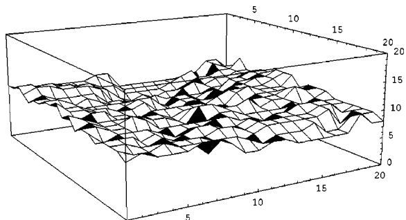
FIG. 6. One of the two interfaces of the slab state on a cubic lattice of linear dimension 20. Coordinates are in units of lattice spacing.
